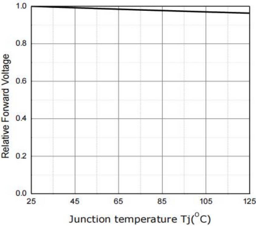
Fig 7. Junction Temperature vs. Relative Forward Voltage, IF=65mA/150mA
