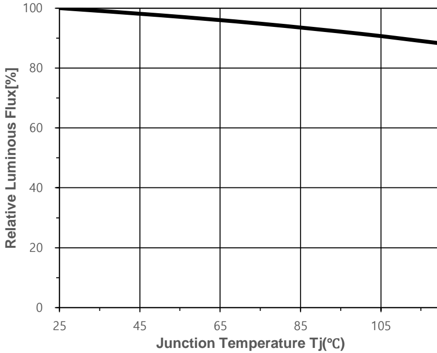
Fig 6. Junction Temperature vs. Relative Luminous Flux, I_F=65\text{mA}
