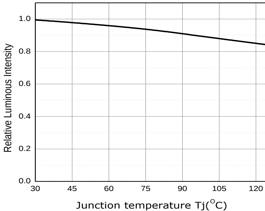
Fig 6. Junction Temperature vs. Relative Luminous Intensity, I_F=65\text{mA}
